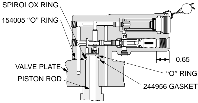
SECTION Y-Y
